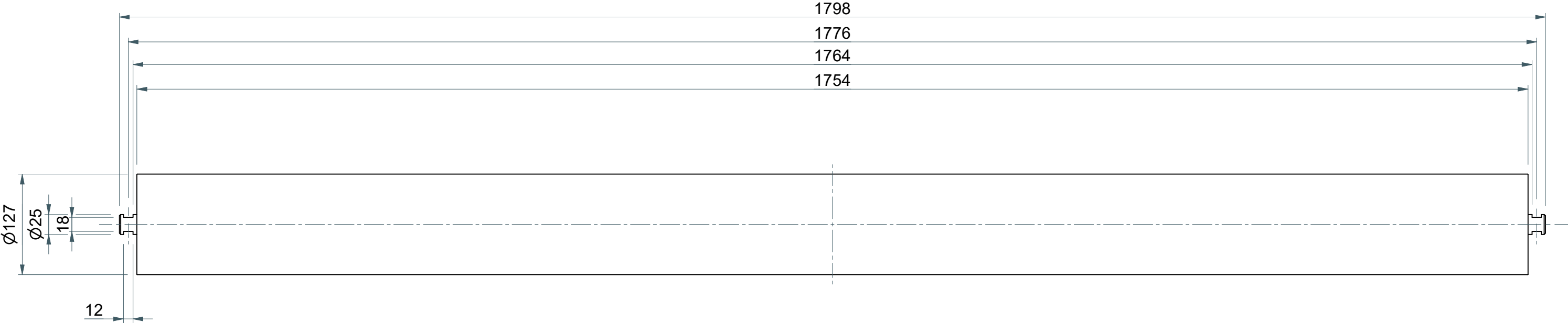
PLAN VIEW SCALE: 1 : 5
