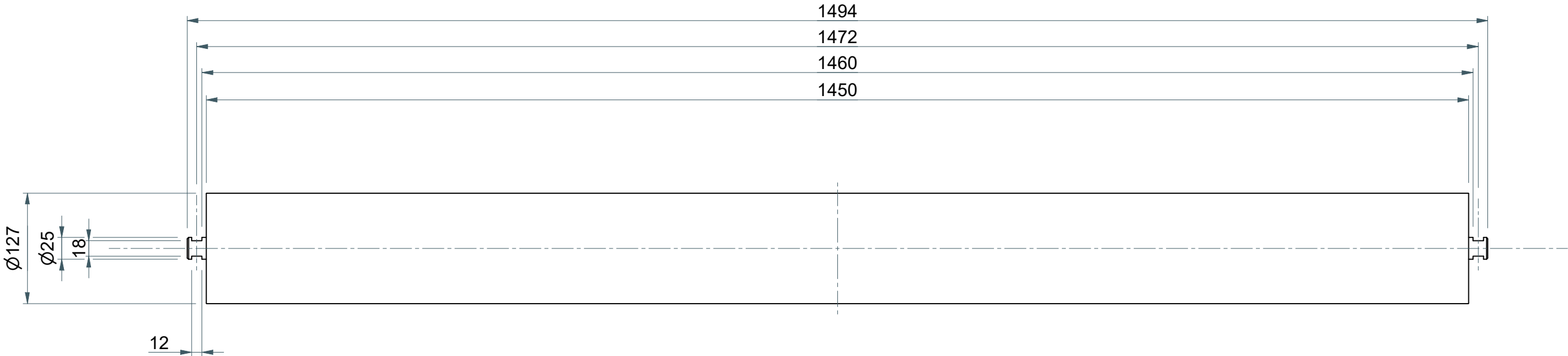
PLAN VIEW SCALE: 1 : 5
